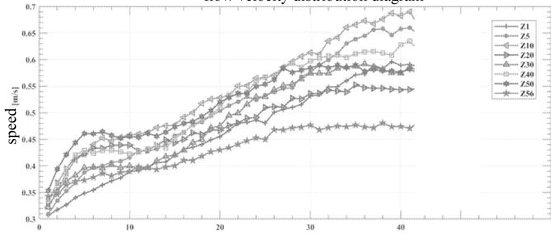
flow velocity distribution diagram
