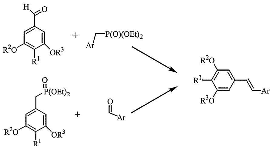
Scheme 1. Wittig olefination:
