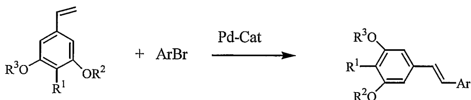
Scheme 2. Heck reaction:
