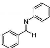
Imine A
