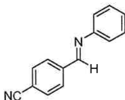
Cyano-imine B
