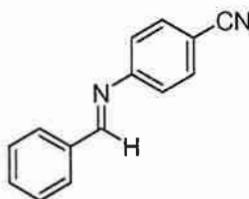
Cyano-imine C
