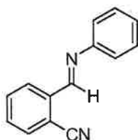
Cyano-imine A
