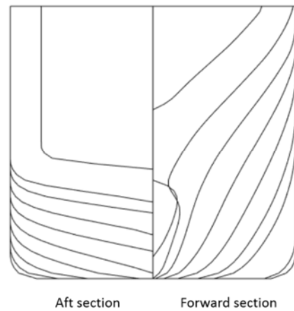
Ship 11 – Cable-laying Ship
