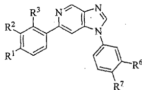
Formula VIa
