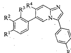
Formula IVb
