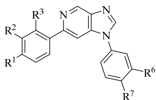
Formula VIa
