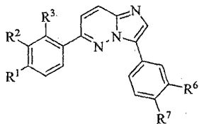
Formula IIIa
