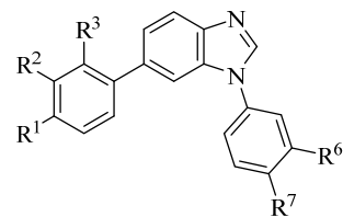
Formula VIIa
