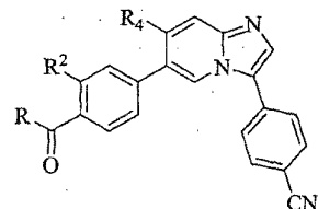
Formula IVc
