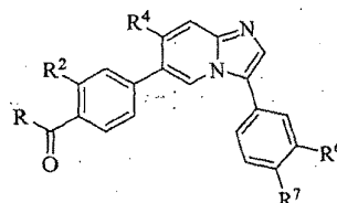
Formula IVa-i
