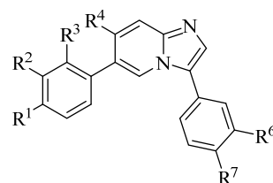
Formula IVa
