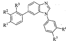
Formula VIIa
