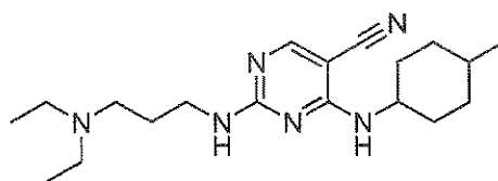
2-(3-(diethylamino)propylamino)-4-(4-methylcyclohexylamino)pyrimidine-5-carbonitrile
