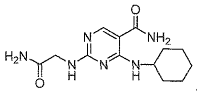
2-(2-aminoethylamino)-4-(cyclohexylamino)pyrimidine-5-carboxamide
