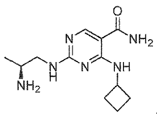
(S)-2-(2-aminopropylamino)-4-(cyclobutylamino)pyrimidine-5-carboxamide
