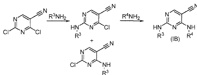
Scheme 8
