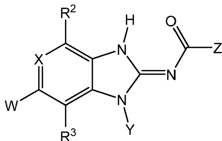
Tautomer A
