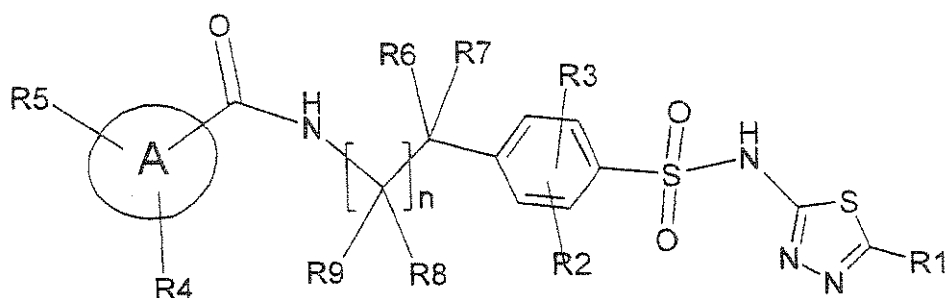
formula I
