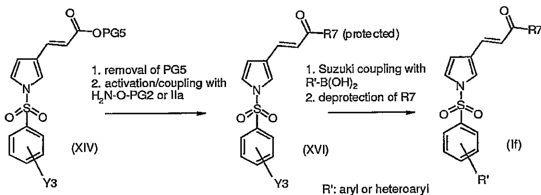
Reaction scheme 7:
