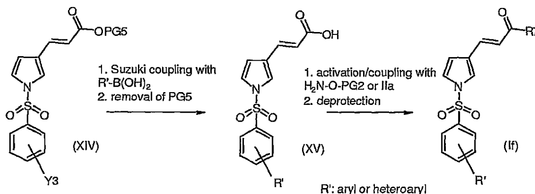
Reaction scheme 6:
