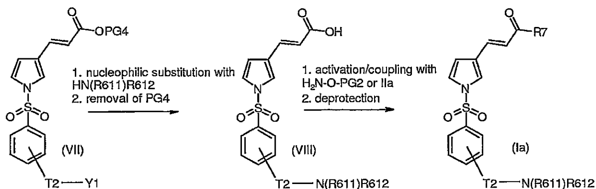
Reaction scheme 2:
