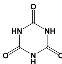
Formula (IIb) (isocyanuric acid)
