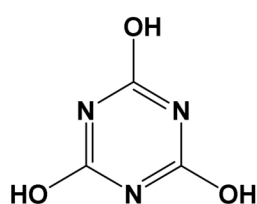
Formula (IIa) (cyanuric acid)
