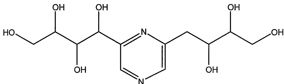
1-[6-(2,3,4-trihydroxybutyl)-pyrazin-2-yl]-butane-1,2,3,4-tetraol (2,6-deoxyfructosazine)
