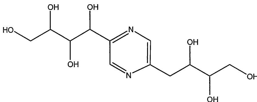
1-[5-(2,3,4-trihydroxybutyl)-pyrazin-2-yl]-butane-1,2,3,4-tetraol 15 (2,5-deoxyfructosazine)
