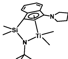
Catalyst 2 Single-chain catalyst
