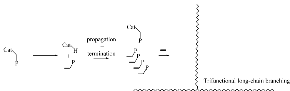
Scheme 1: Naturally occurring long-chain branching: Chain transfer event leading to vinyl terminated polymers
