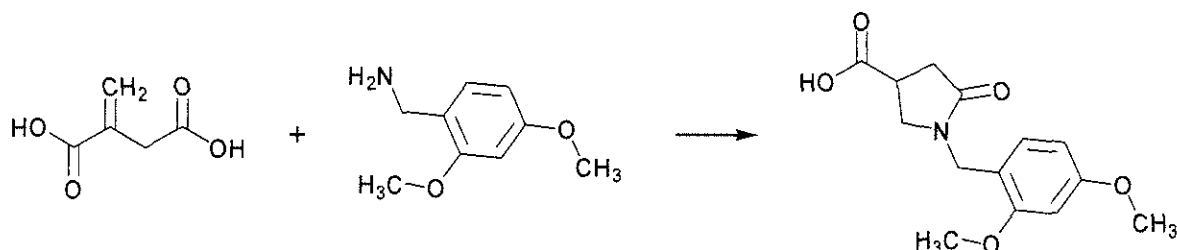
(1) 1-(2,4-Dimethoxybenzyl)-5-oxopyrrolidine-3-carboxylic acid
