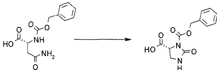
(1) (R)-2-Oxoimidazolidine-1,5-dicarboxylic acid 1-benzyl ester
