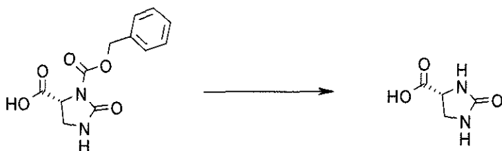
(2) (R)-2-Oxoimidazolidine-4-carboxylic acid
