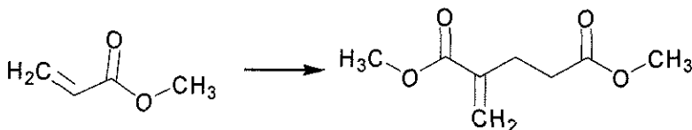
(1) 2-Methylenepentanedioic acid dimethyl ester
