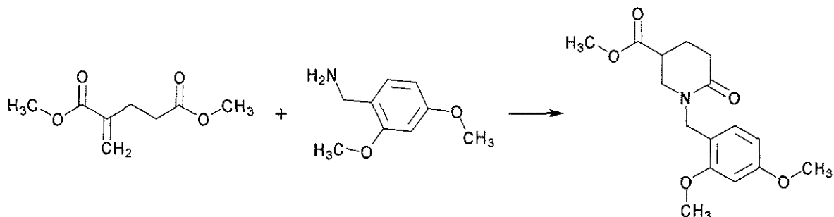
(2) 1-(2,4-Dimethoxybenzyl)-6-oxopiperidine-3-carboxylic acid methyl ester
