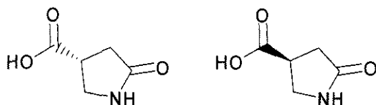
(1) 1-(2,4-Dimethoxybenzyl)-5-oxopyrrolidine-3-carboxylic acid
