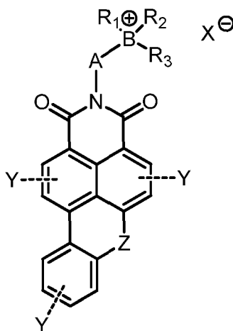
(Formula I)
