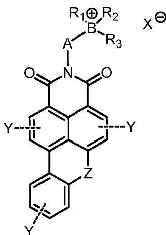
(Formula I)
