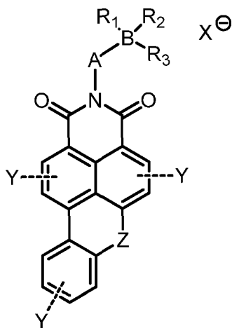
Formula I
