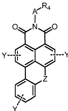
Formula II
