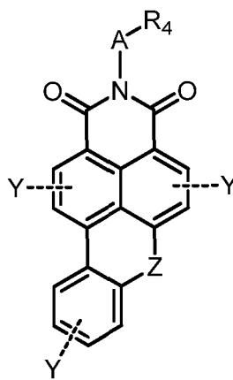
Formula II
