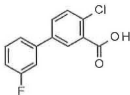
2-Chloro-5-(3-fluorophenyl)benzoic acid (intermediate III(g))
