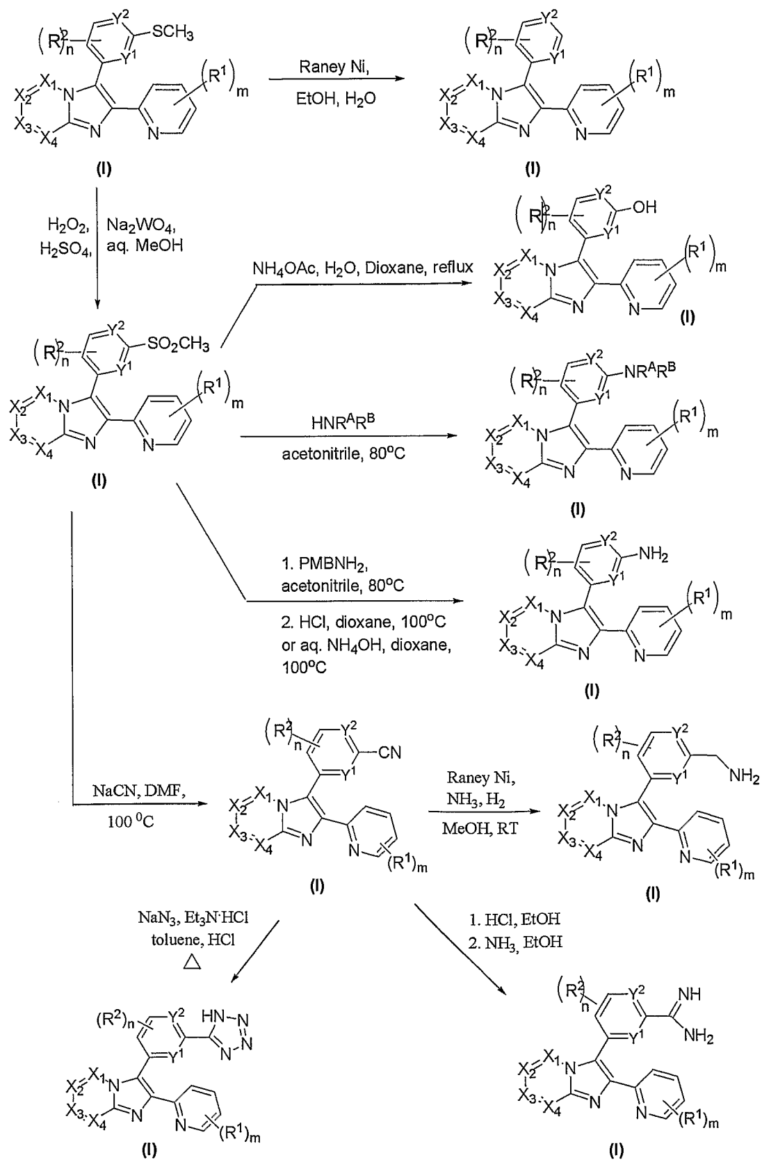
Scheme 2
