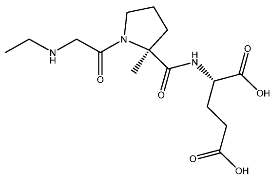
(IIIa) Et-Gly-MePro-Glu-OH,
