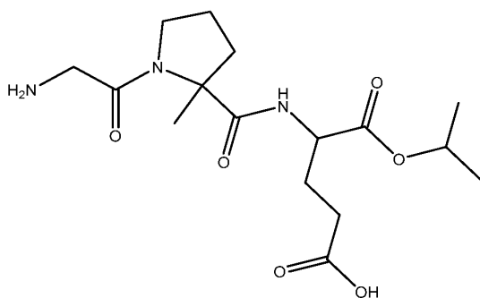
(VII) (Gly-MePro-Glu-OiPr),
