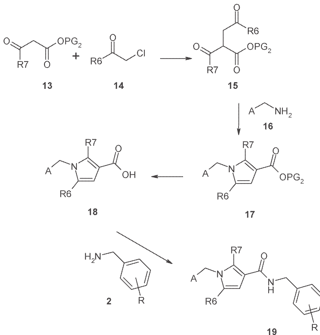
Scheme 3
