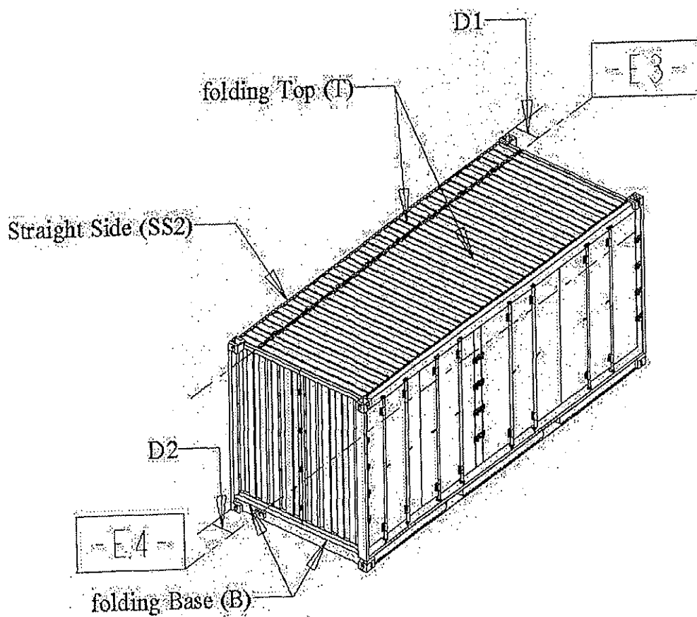
Figure 4 The folding edges in the surface B and surface T of the folding container
