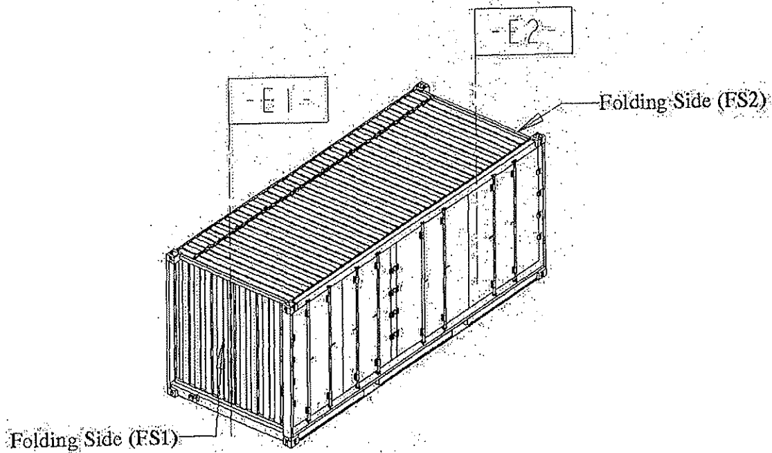
Figure 2 Folding sides FS1 and FS2 of folding container.
