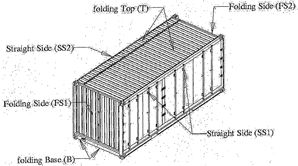
Figure 1 Schematic diagram of a folding container
