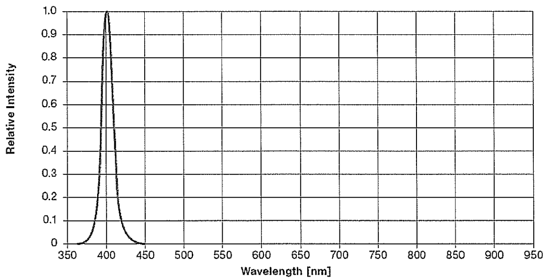
Figure 2/2: Spectrum of the UV-LED
