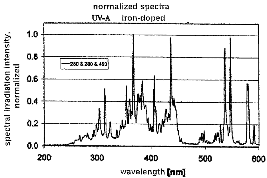
Figure 1/2: Hönle exposure device:
