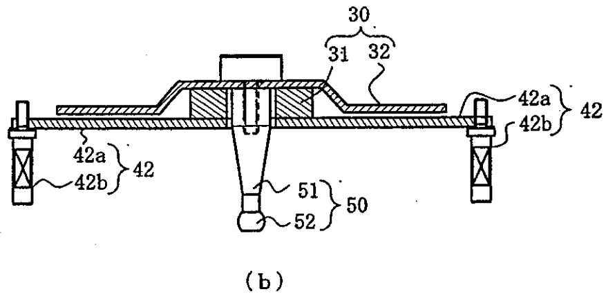
B-B CROSS SECTION
