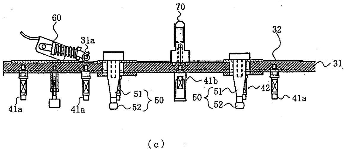
C-C CROSS SECTION
