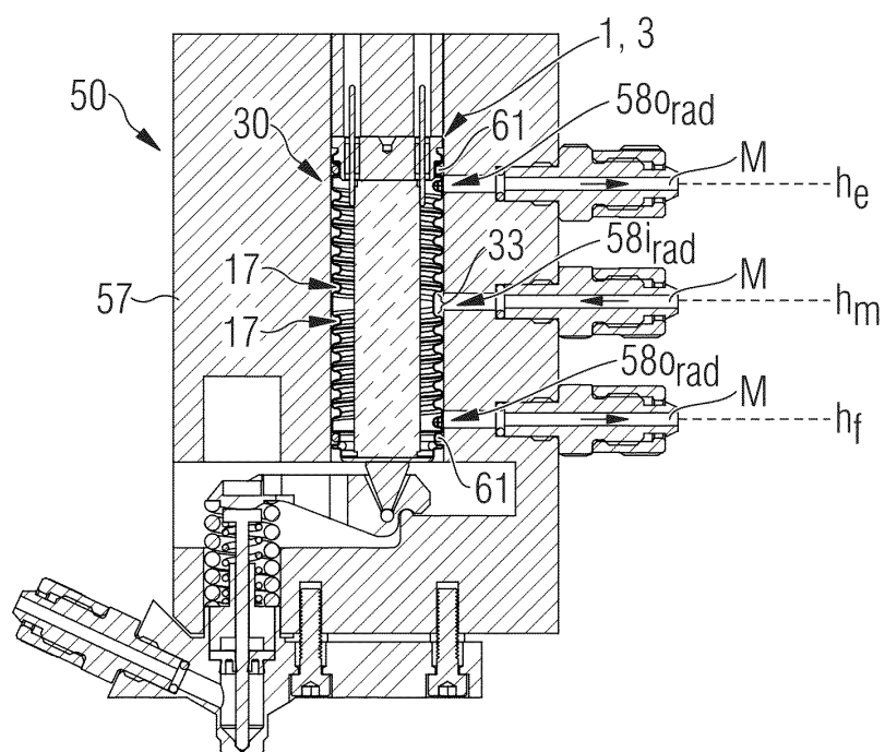
FIG 6 A''-A''
