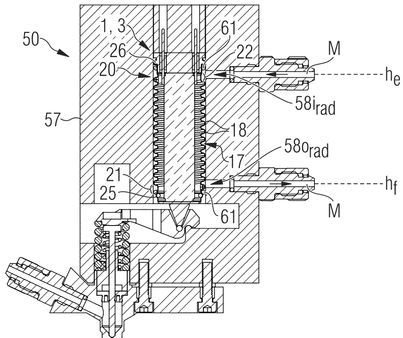
FIG 4 A'-A'
