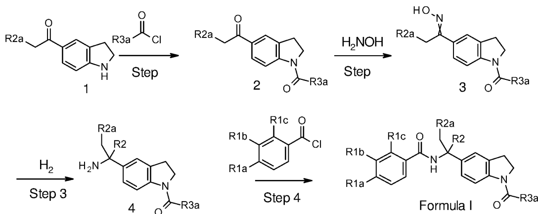
Scheme 1: Synthesis of compounds of Formula I
