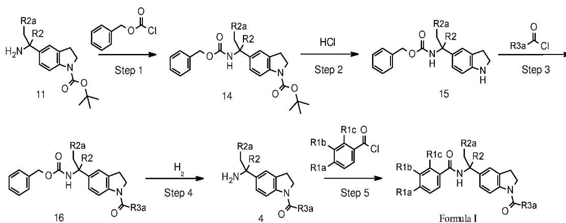
Scheme 4: Synthesis of compounds of Formula I
