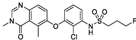
N-(2-chloro-3-((3,5-dimethyl-4-oxo-3,4-dihydroquinazolin-6-yl)oxy)phenyl)-3-fluoropropane-1-sulfonamide
