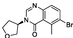
(R)-6-bromo-5-methyl-3-(tetrahydrofuran-3-yl)quinazolin-4(3H)-one
