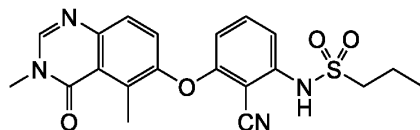
N-{2-Cyano-3-[(3,5-dimethyl-4-oxo-3,4-dihydroquinazolin-6-yl)oxy]phenyl}propane-1-sulfonamide
