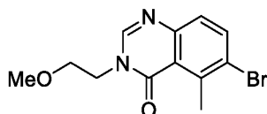
6-bromo-3-(2-methoxyethyl)-5-methylquinazolin-4(3H)-one
