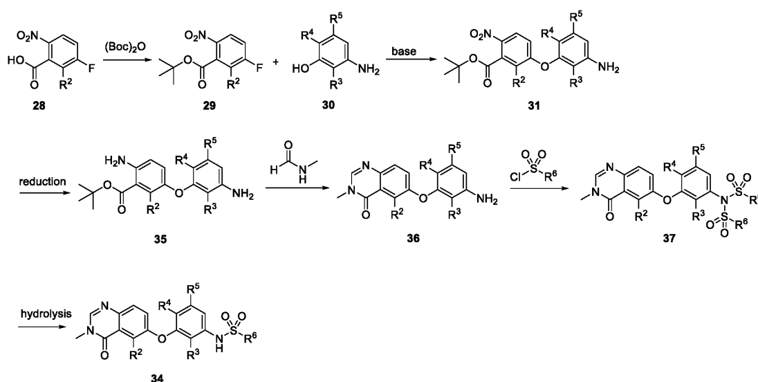
Scheme 12
