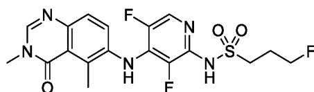
N -(4-((3,5-dimethyl-4-oxo-3,4-dihydroquinazolin-6-yl)amino)-3,5-difluoropyridin-2-yl)-3-fluoropropane-1-sulfonamide
