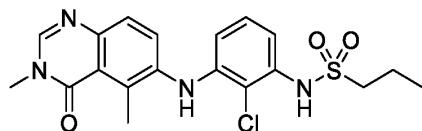
N -(2-chloro-3-((3,5-dimethyl-4-oxo-3,4-dihydroquinazolin-6-yl)amino)phenyl)propane-1-sulfonamide
