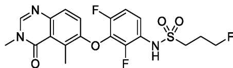
N-(3-((3,5-dimethyl-4-oxo-3,4-dihydroquinazolin-6-yl)oxy)-2,4-difluorophenyl)- 3-fluoropropane-1-sulfonamide
