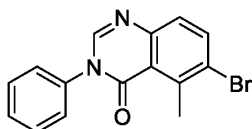
6-bromo-5-methyl-3-phenylquinazolin-4(3H)-one
