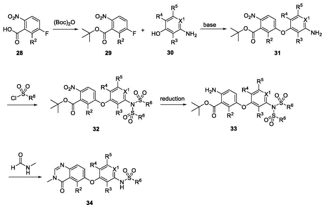
Scheme 11
