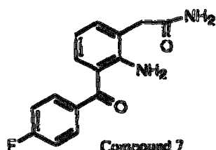
Compound 7
