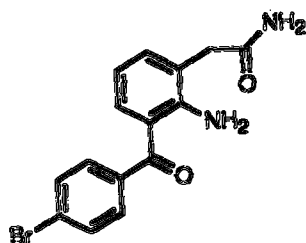
Compound 15 2-Amino-3-(4-bromobenzoyl)-phenylacetamide
