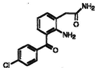
Compound 9 2-Amino-3-(4-chlorobenzoyl)-phenylacetamide
