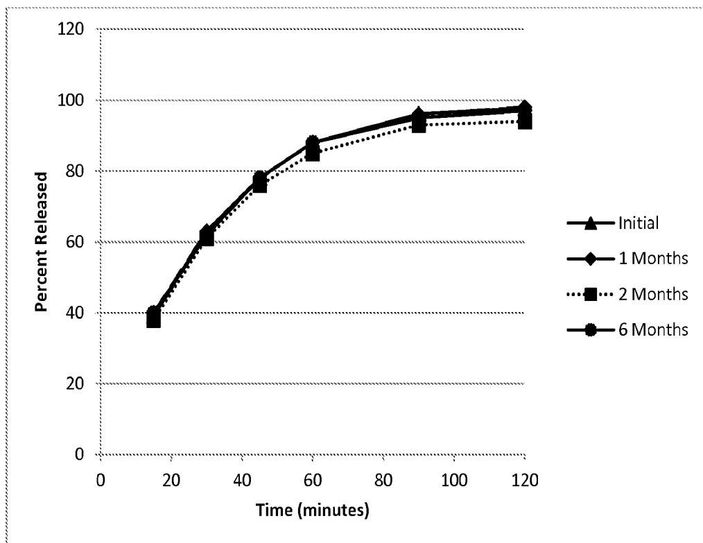
Figure 3. Average Dissolution of 4g Chewables Stored at 25°C/60%RH
