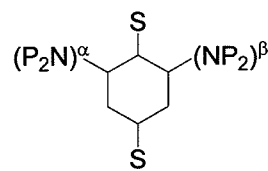
Structure AI
