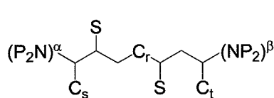
Structure AD
