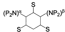
Structure AL
