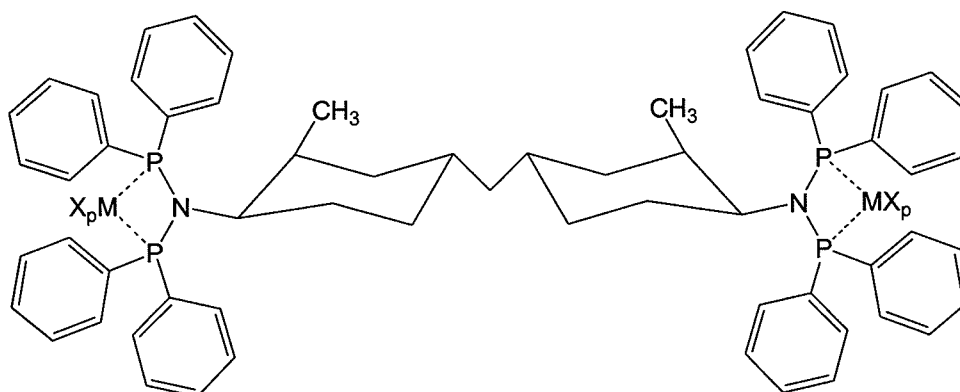
Structure XVIII
