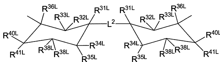
Structure 10L
