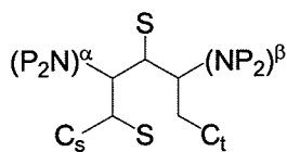
Structure AH
