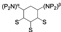
Structure AK
