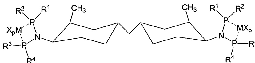
Structure XVI
