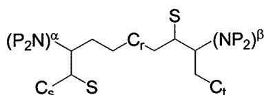
Structure AQ
