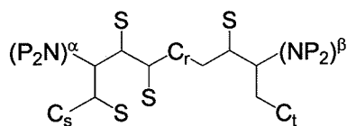
Structure AG
