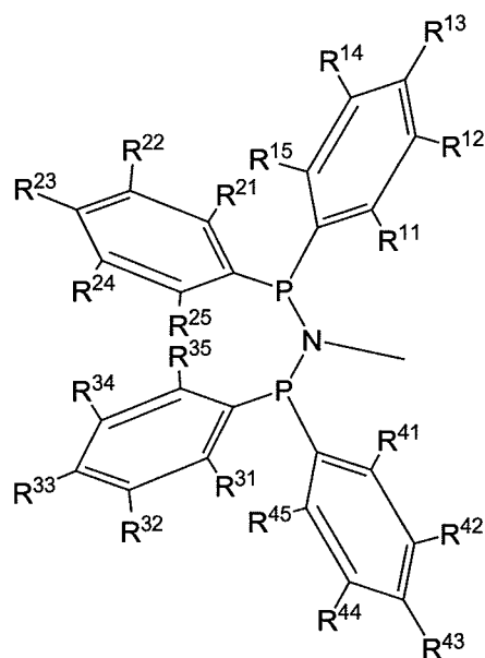
Structure 3
