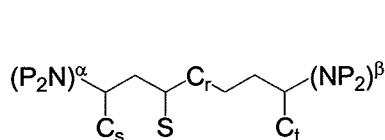
Structure AA
