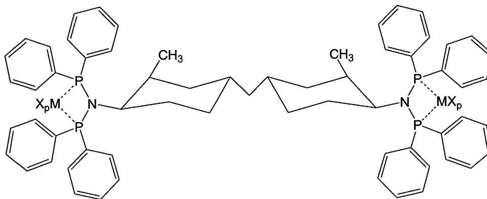
Structure XVIII
