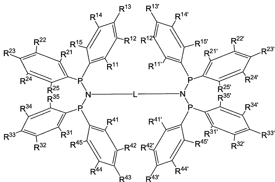
Structure V
