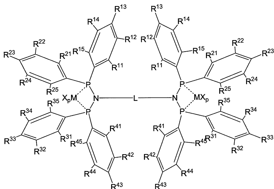
Structure XIV
