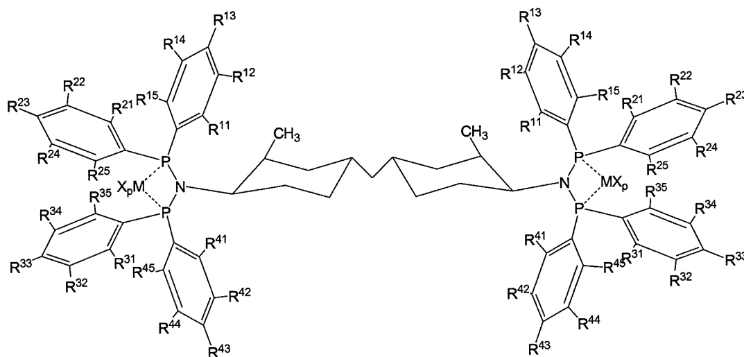
Structure XVII
