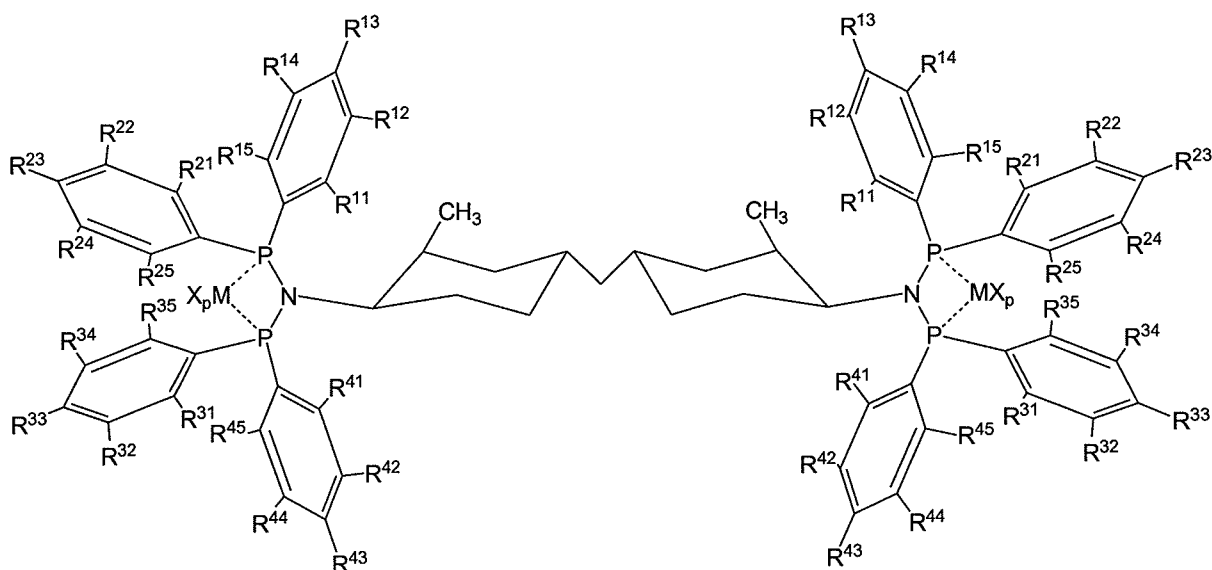
Structure XVII
