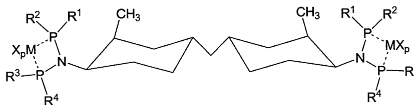
Structure XVI
