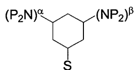
Structure AB
