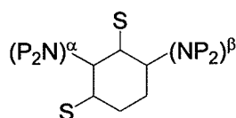
Structure AJ
