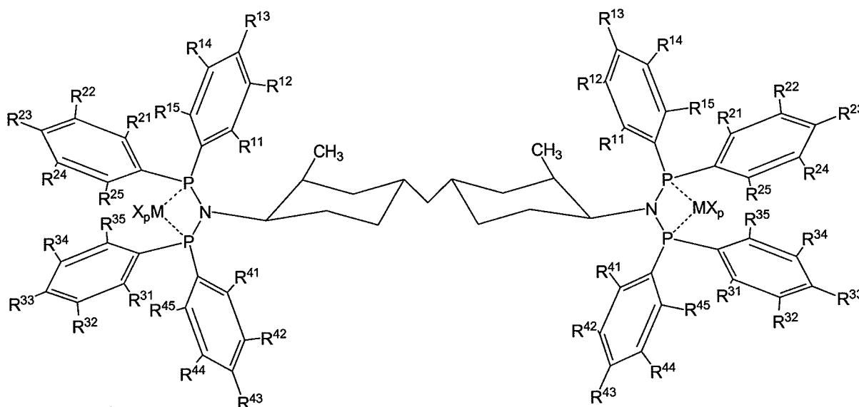
Structure XVII
