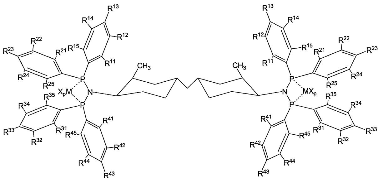
Structure XVII
