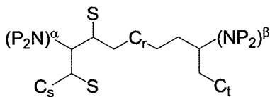
Structure AE
