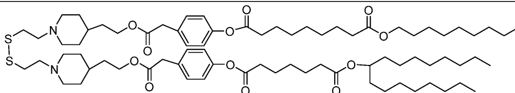
Lipid 18
