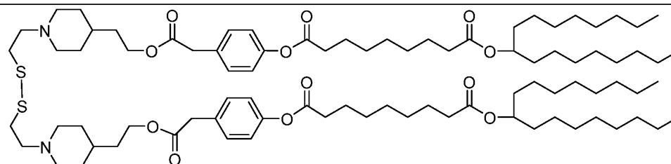
Lipid 5
