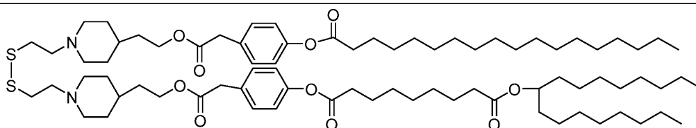
Lipid 14
