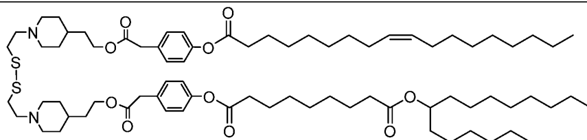
Lipid 8
