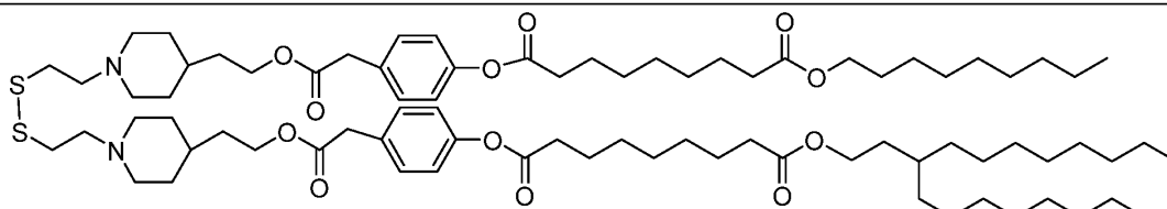
Lipid 19
