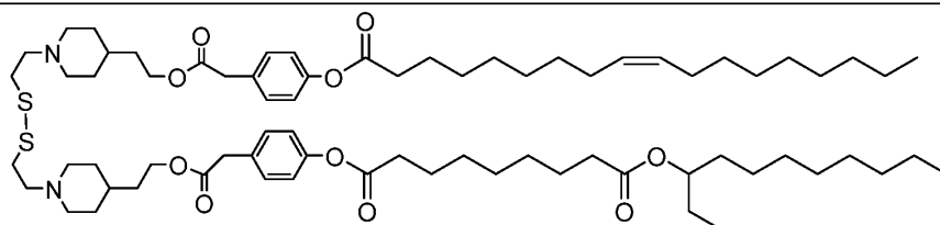
Lipid 6
