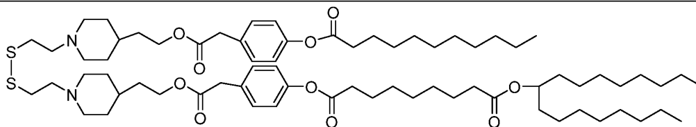
Lipid 15
