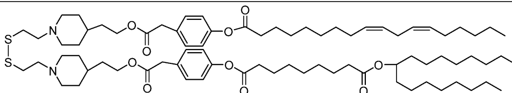
Lipid 12
