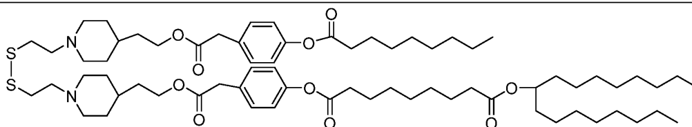
Lipid 16
