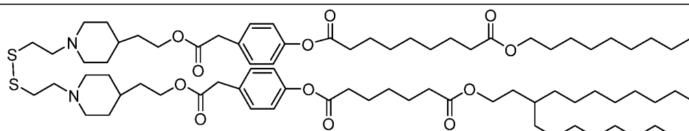
Lipid 20
