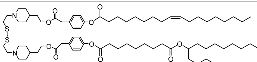
Lipid 7
