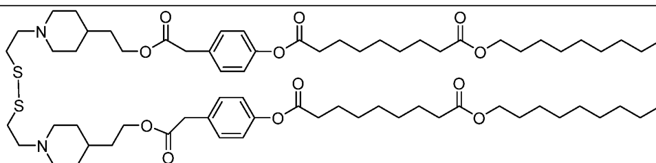
Lipid 4
