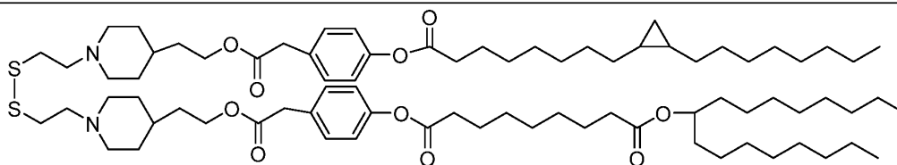
Lipid 13
