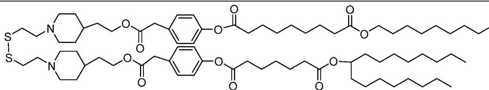
Lipid 17
