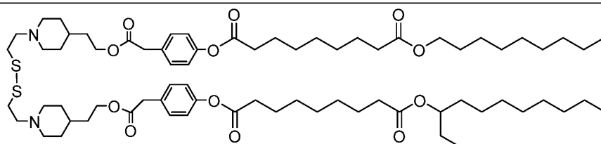
Lipid 9
