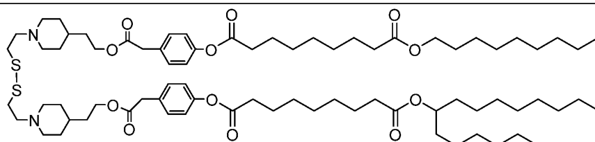
Lipid 11
