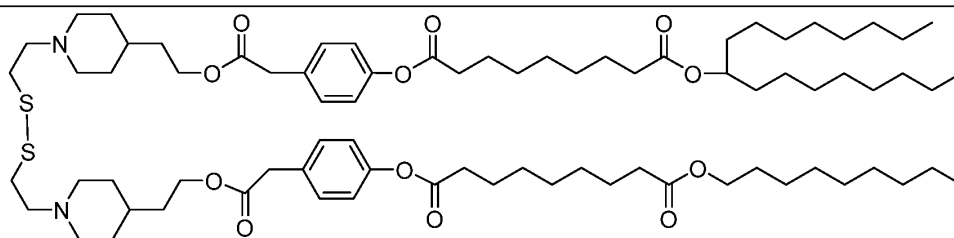
Lipid 3
