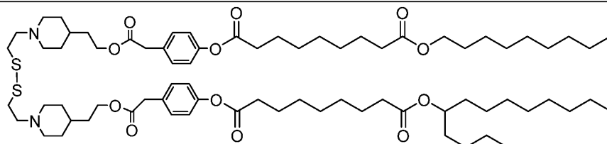
Lipid 10
