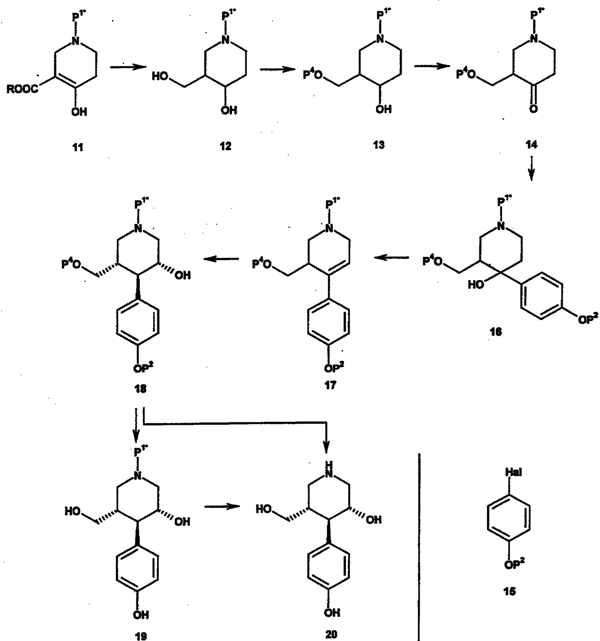
Scheme 3:
