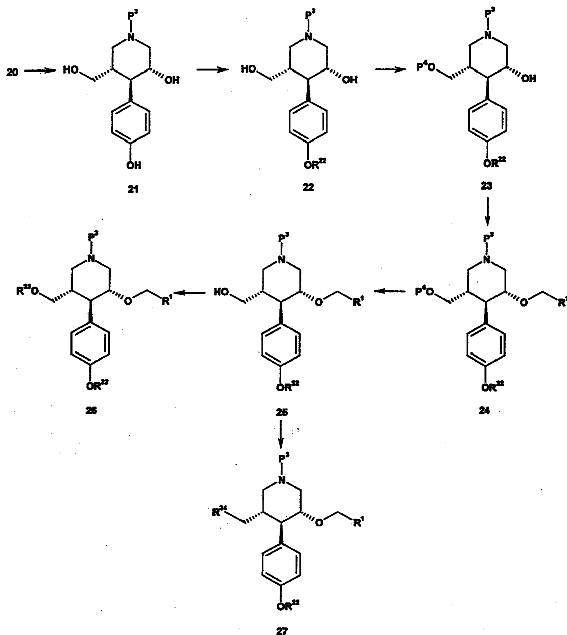
Scheme 4:
