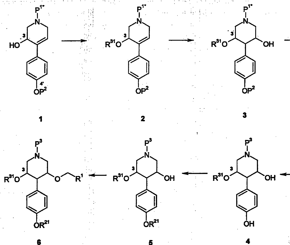
Scheme 1:
