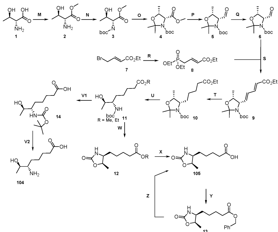
Scheme 1. Synthetic route and procedures for Compounds 104 , 105 , 106 , 114 and 115 .
