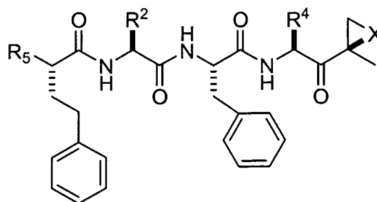
(XII)
