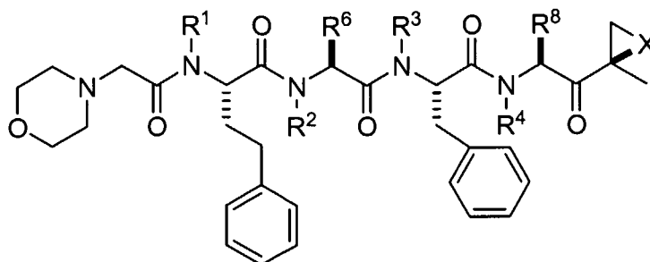
(X)
