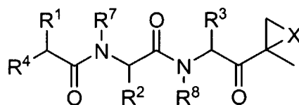
(XIII)
