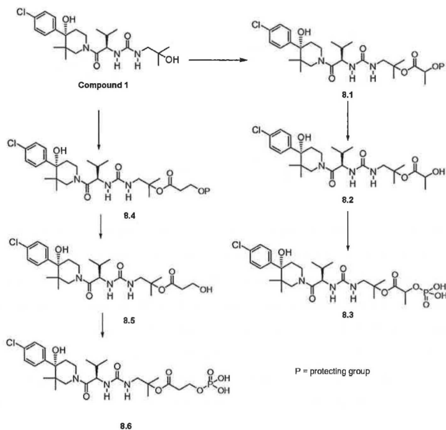
Scheme 8
