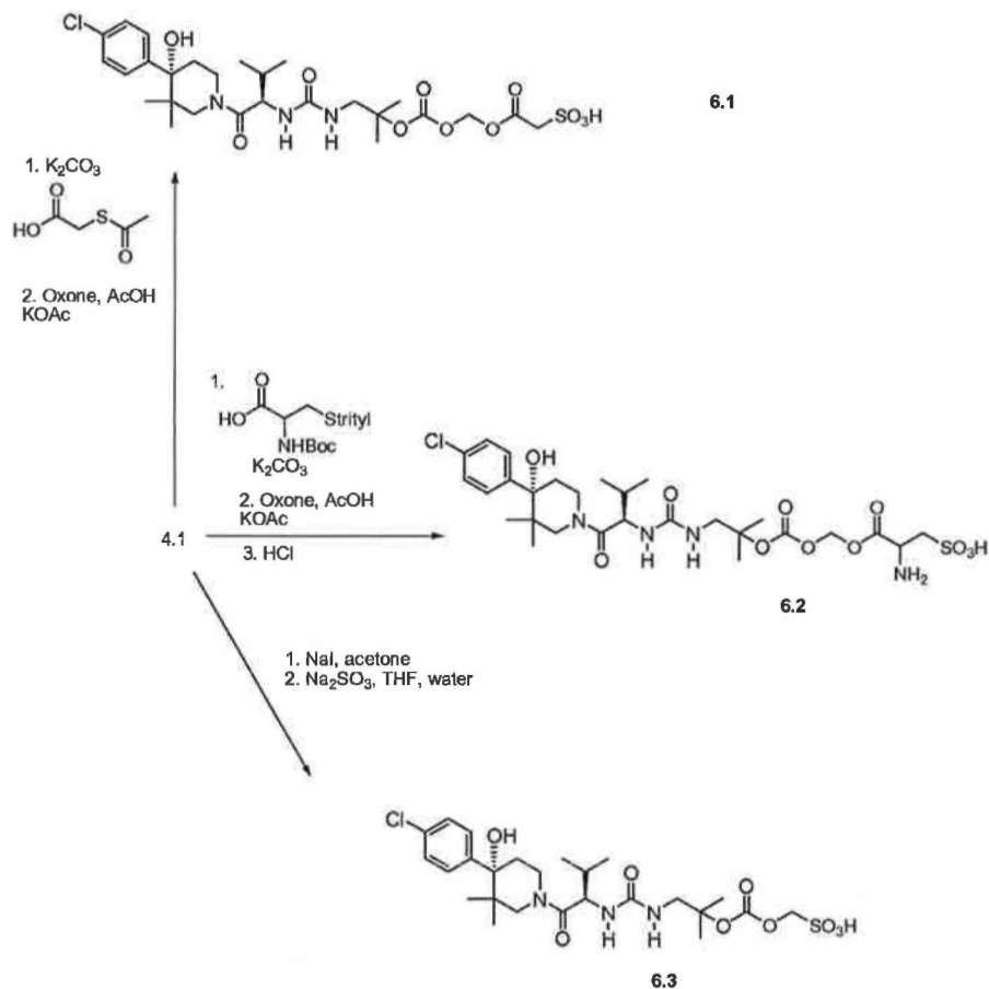
Scheme 6
