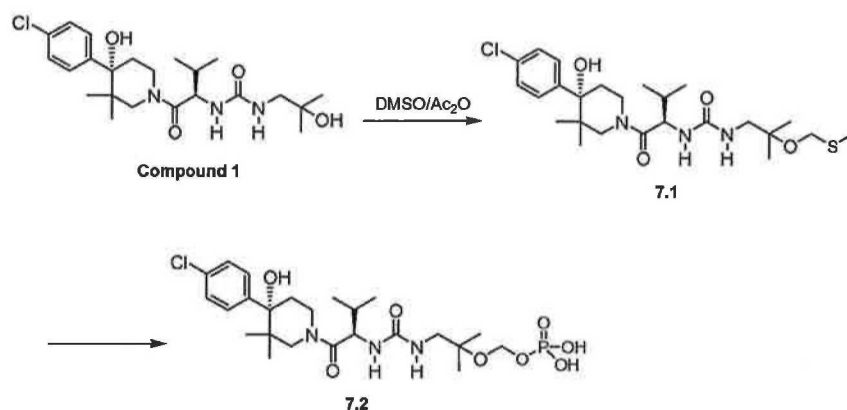
Scheme 7
