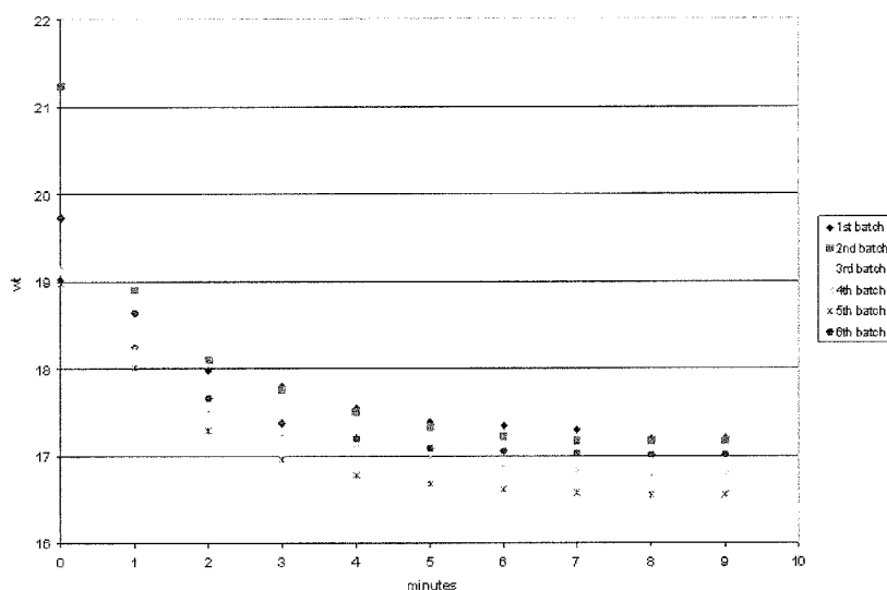
Figure 1 Graph of Drying of Molecular Sieves after they have removed moisture from coal fines
