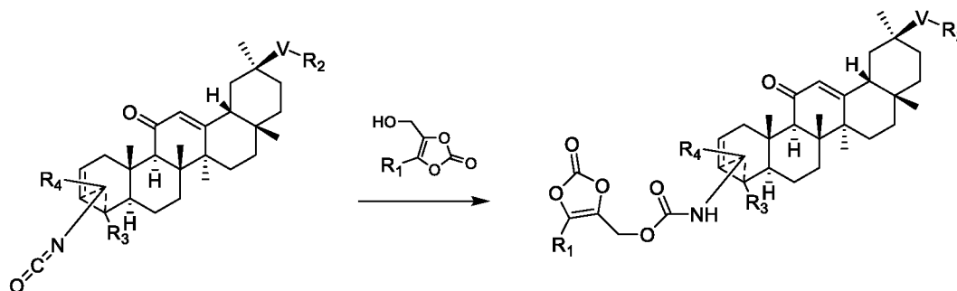
Scheme 3
