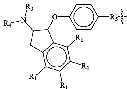
(XII-H)
