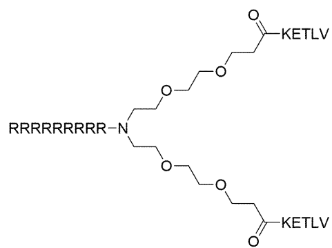
Formula (X)
