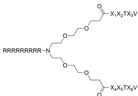
Formula (IX)
