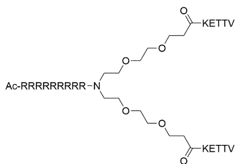
Formula (XVIII)
