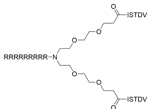
Formula (XIV)
