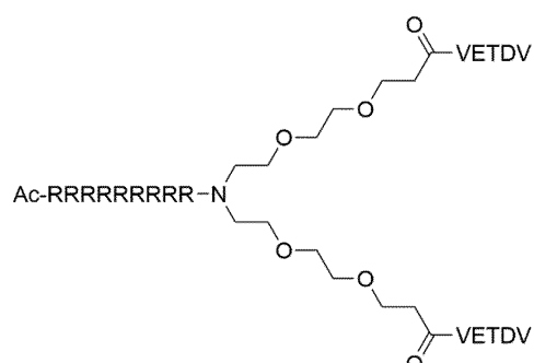
Formula (XX)
