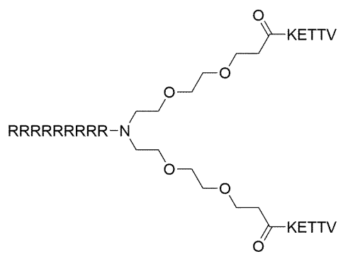
Formula (XI)
