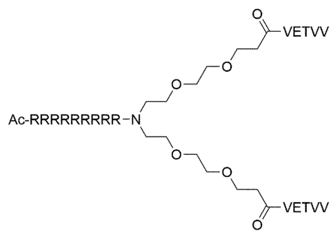
Formula (XXII)
