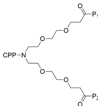
Formula (XXVIII)
