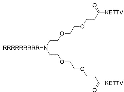
Formula (XI)
