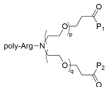
Formula (IV)
