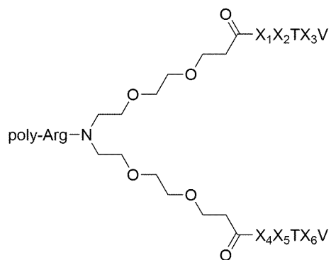
Formula (VIII)
