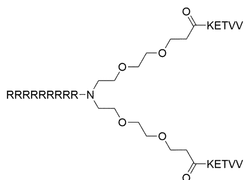
Formula (XII)
