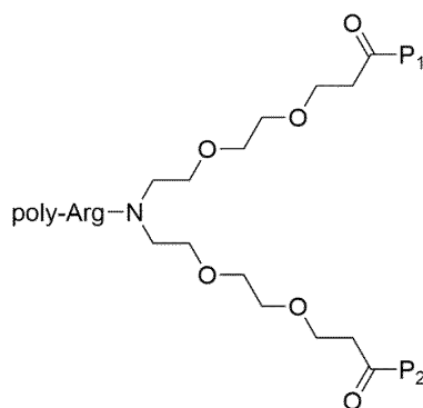
Formula (VII)
