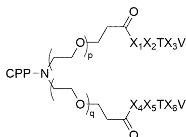
Formula (V)
