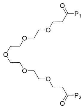
Formula (XXVII)
