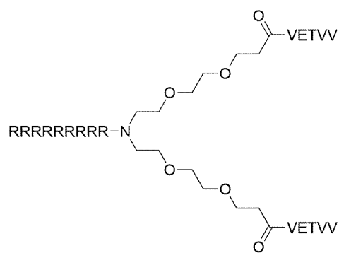
Formula (XV)
