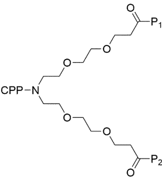
Formula (XXVIII)
