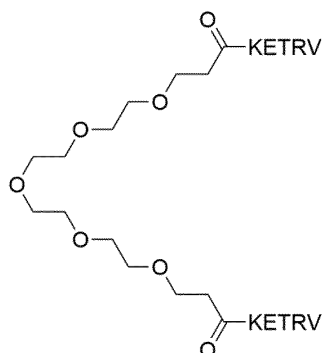
Formula (XXXII)
