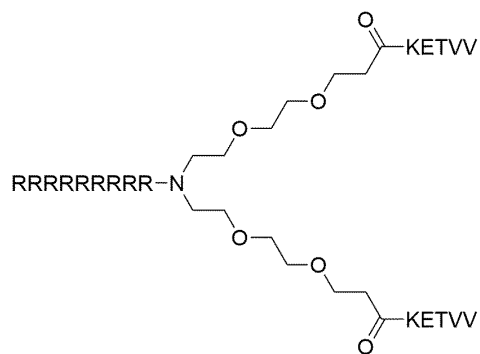
Formula (XII)
