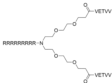
Formula (XV)
