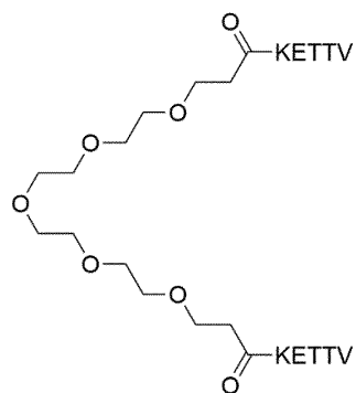
Formula (XXX)
