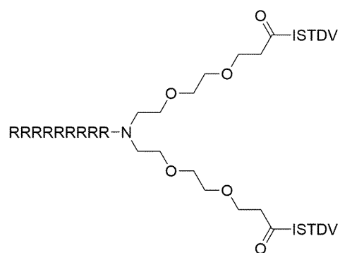
Formula (XIV)
