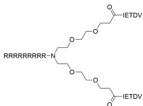
Formula (XVI)
