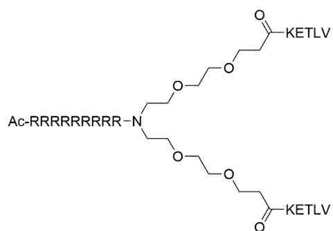
Formula (XVII)
