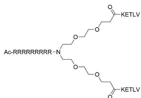
Formula (XVII)
