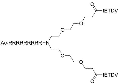
Formula (XXIII)
