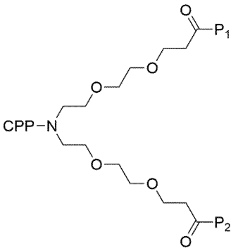
Formula (XXVIII)
