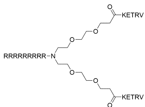
Formula (XIII)
