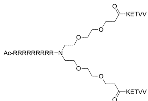
Formula (XIX)
