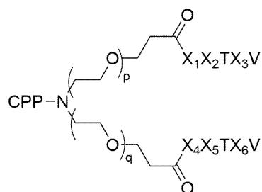
Formula (V)
