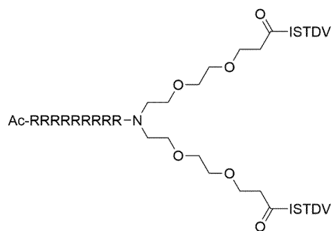
Formula (XXI)
