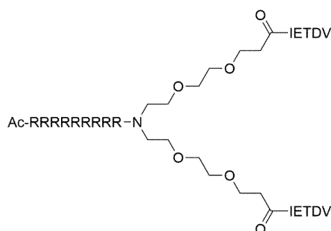
Formula (XXIII)
