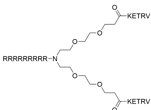
Formula (XIII)
