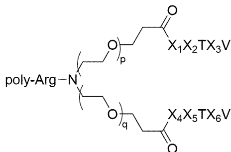
Formula (VI)
