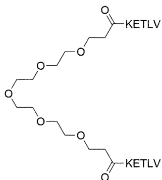
Formula (XXIX)
