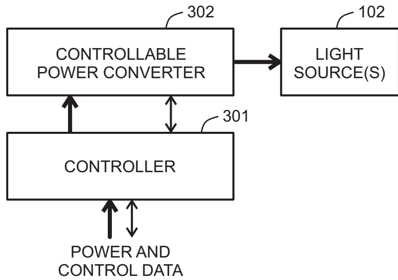
Fig. 3 PRIOR ART
