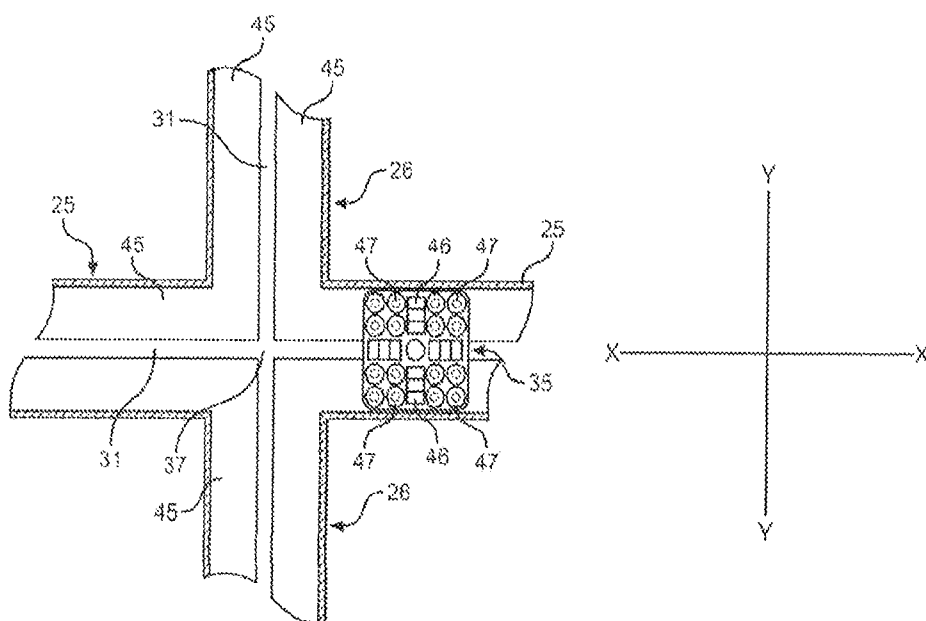
FIG. 5 PRIOR ART
