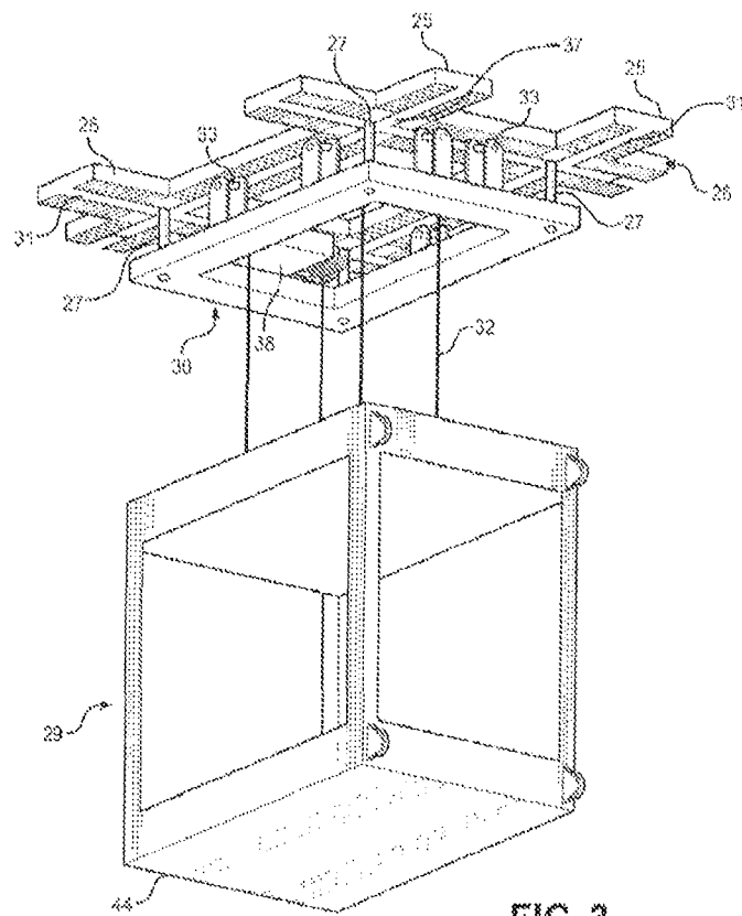
FIG. 3 PRIOR ART
