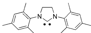
1,3-Bis(2,4,6-trimethylphenyl)-4,5-dihydroimidazol-2-ylidene (Im-7)
