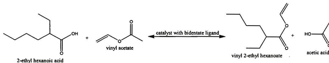
Formula III.
