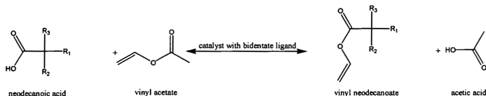
Formula IV.
