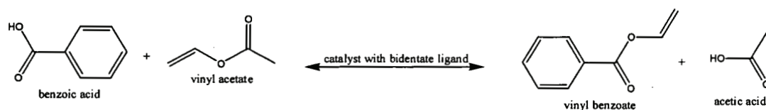
Formula II.
