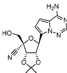
Intermediate I-1a
