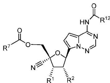
Formula X.
