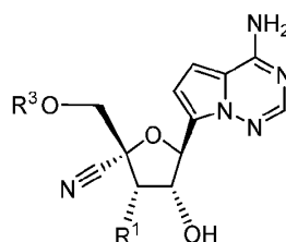
Formula IV.
