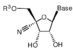
Formula XI.
