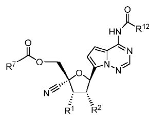
Formula X.
