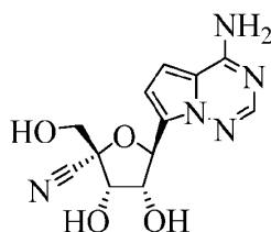
Compound 0
