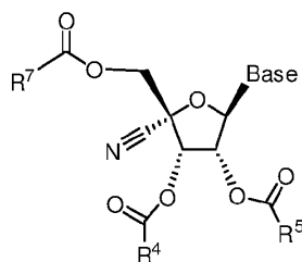
Formula IX.
