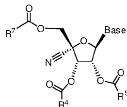
Formula IX.
