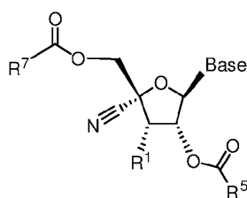
Formula VIII.
