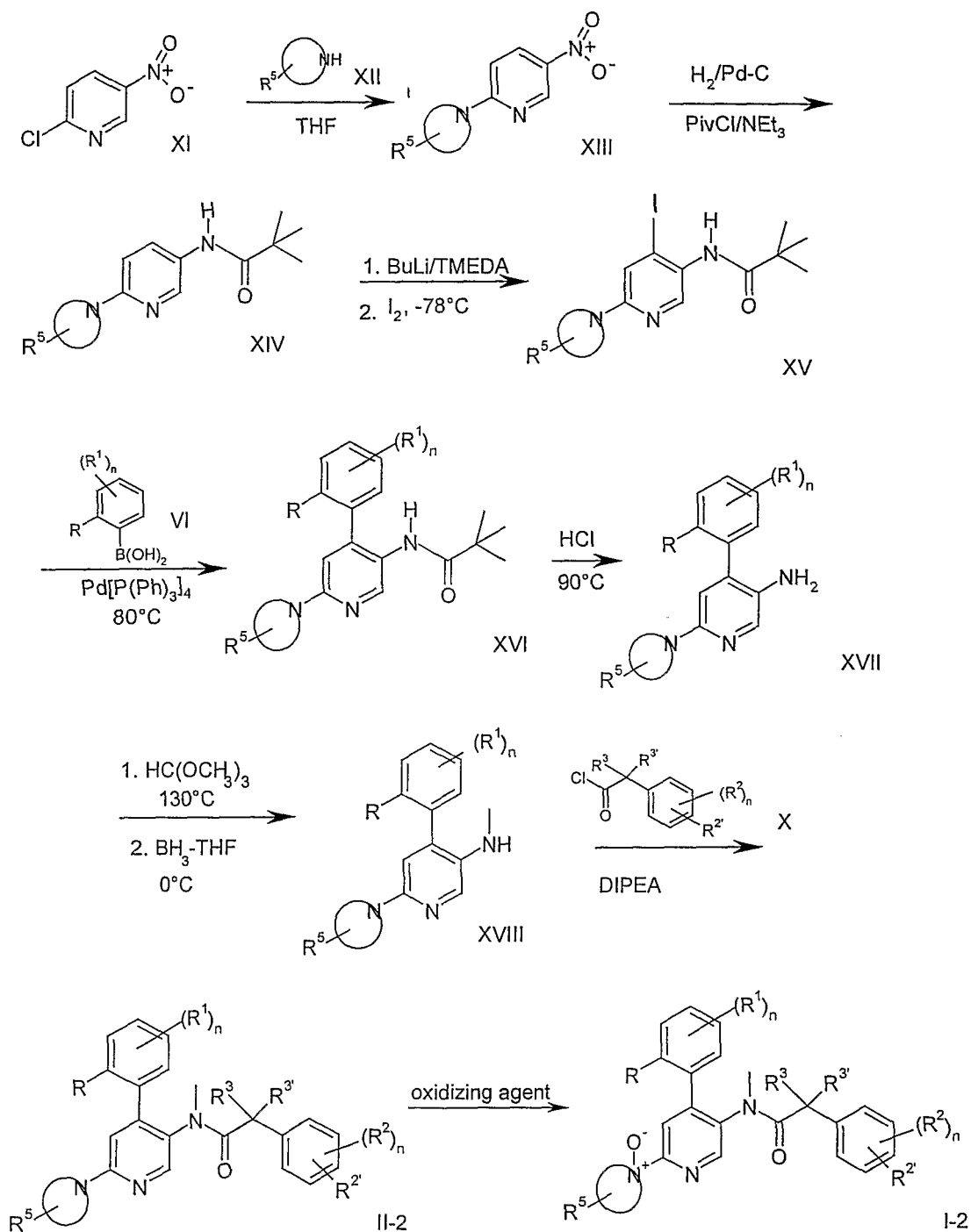
Scheme 2
