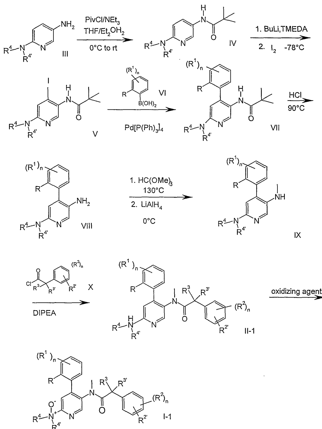
Scheme 1
