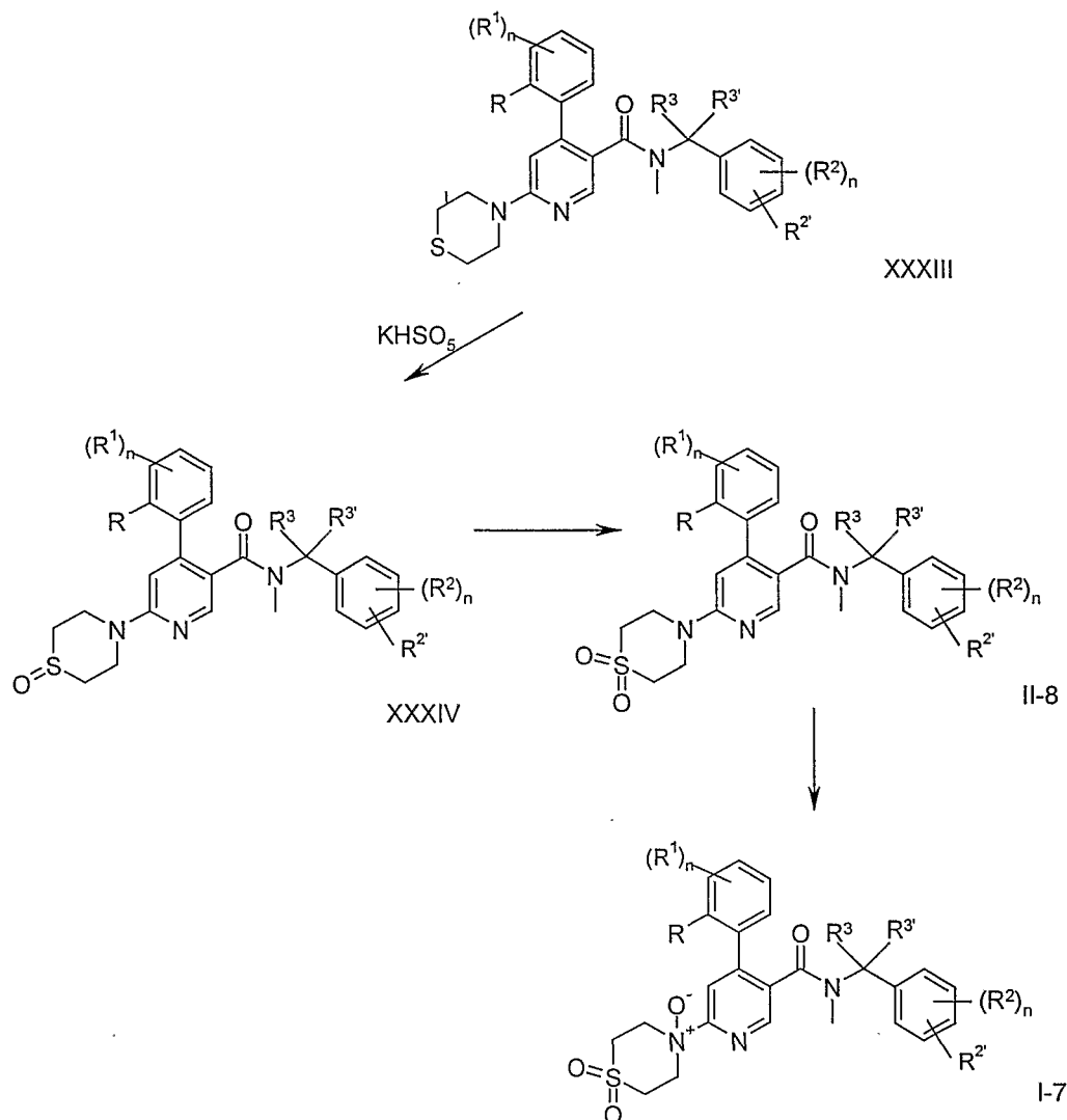
Scheme 8
