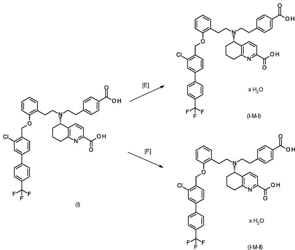
Scheme 3: selective crystallization of the acid of formula (I) to yield monohydrate forms thereof
