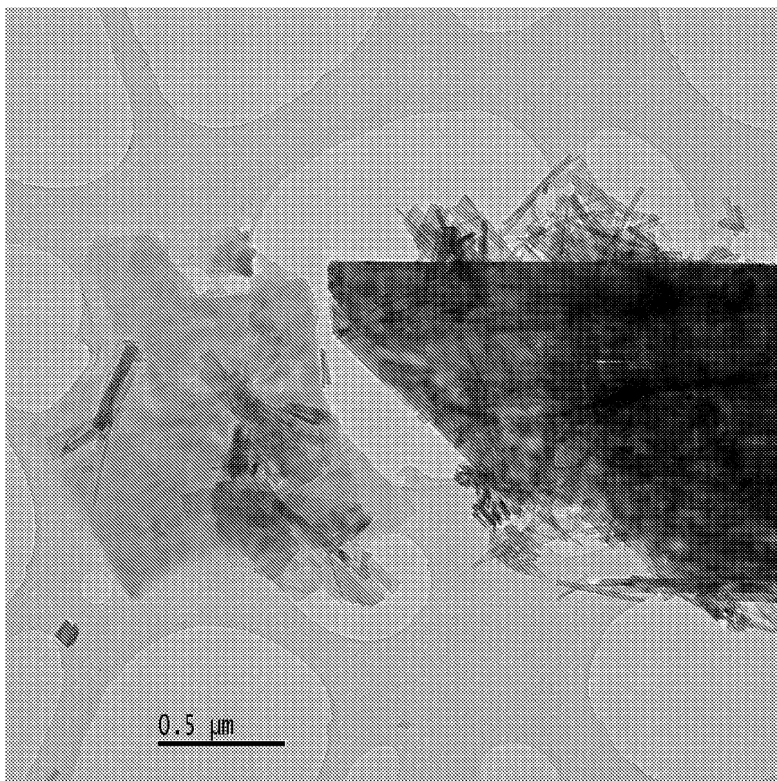
Figure 6 TEM image of example 8 crystals
