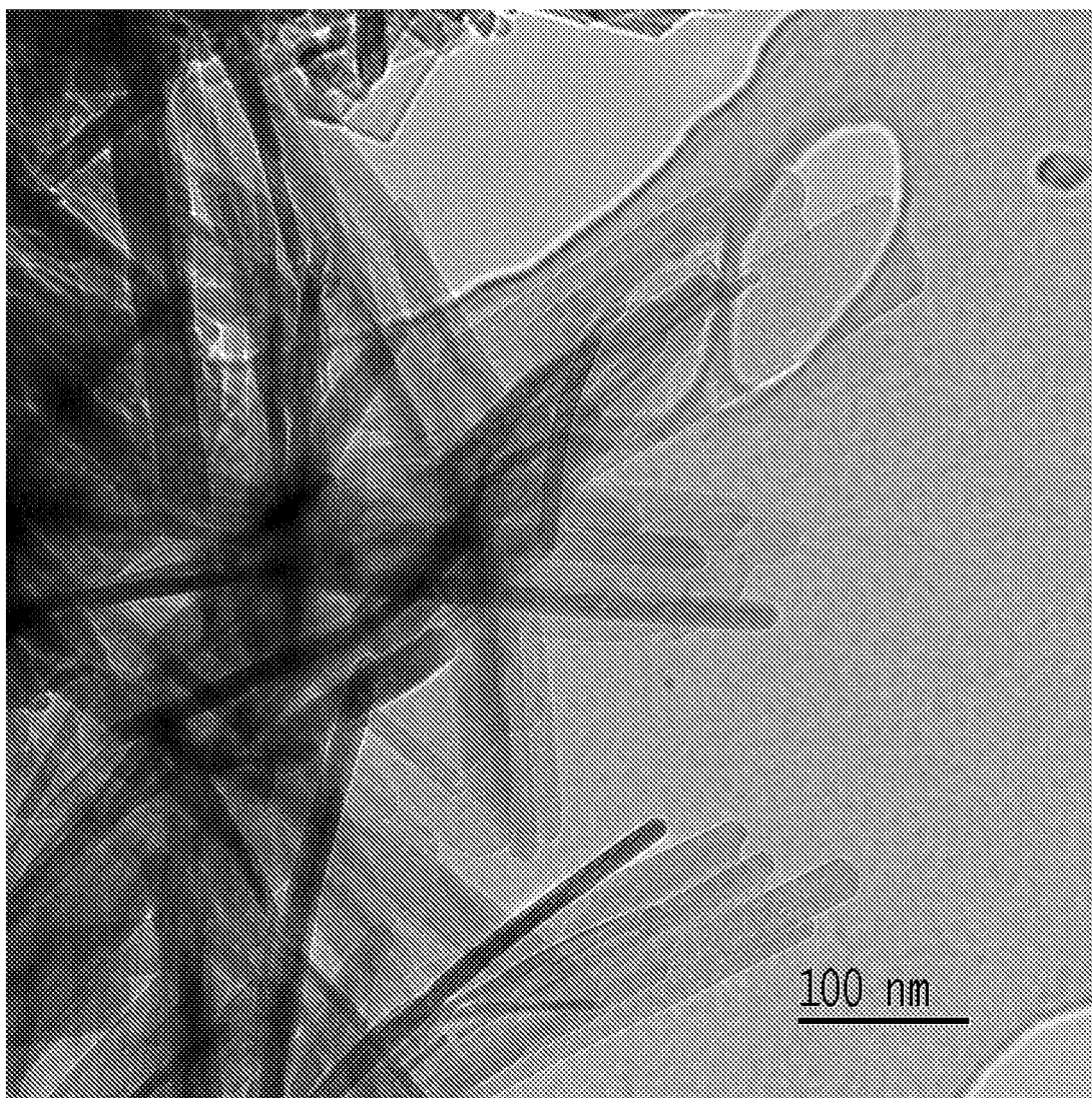
5 Figure 8 TEM Image of Example 11 at 100nm scale showing presence of nano-rods
