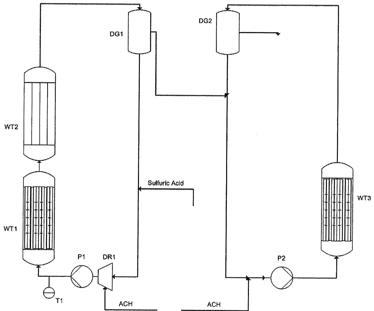
Fig. 3: Flow diagram for examples 1-4
