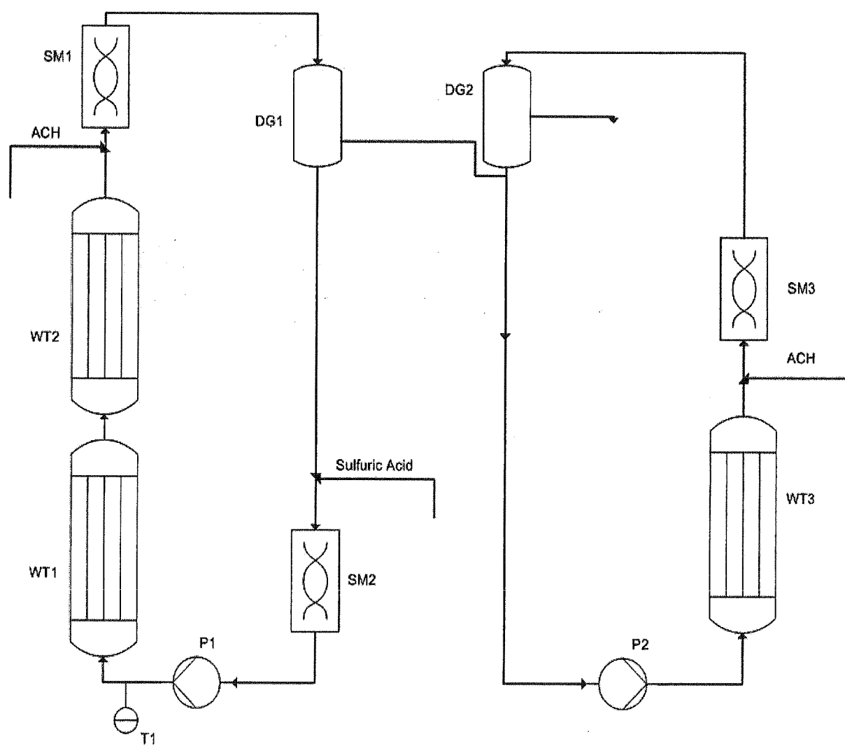
Fig. 2 Flow diagram for comparative examples 1-4
