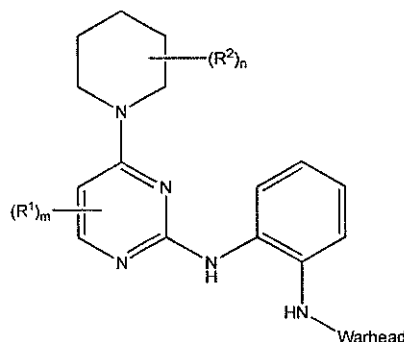
Formula VII
