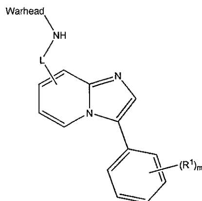
Formula VI
