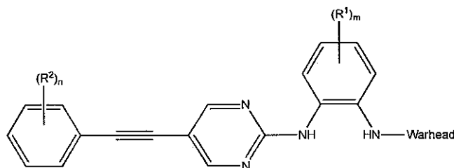
Formula IX
