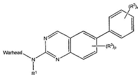
Formula IV
