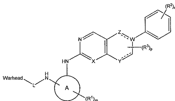
Formula VIII
