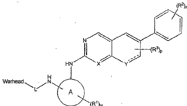
Formula I
