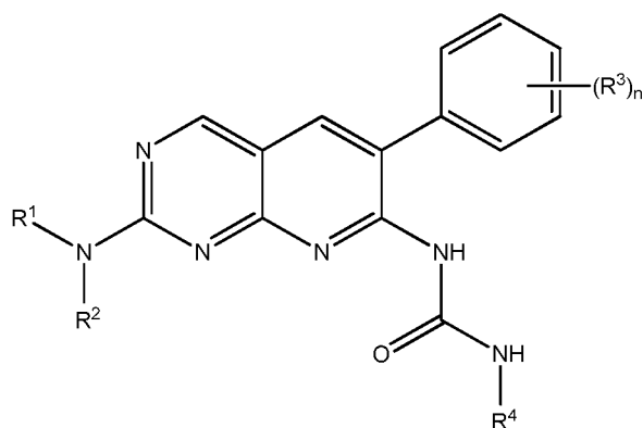
Formula X
