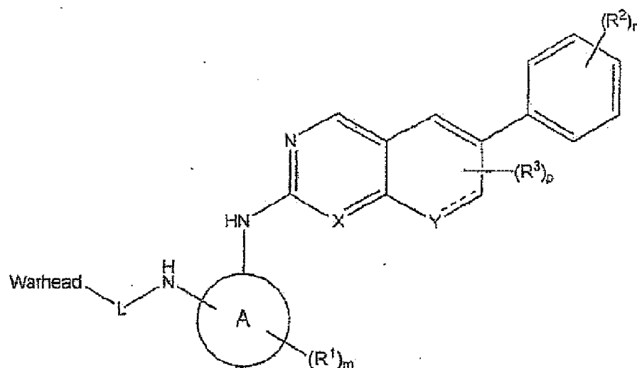
Formula I
