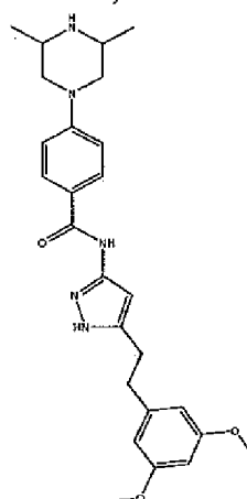
AZD4547
