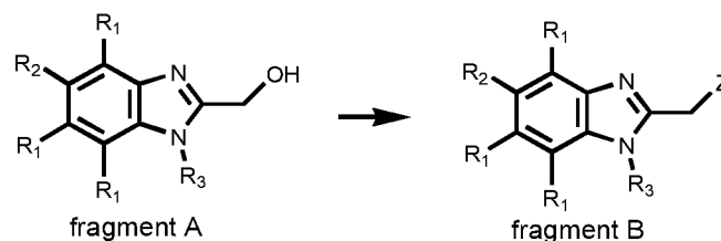
10 Scheme 3. General synthesis of fragment B type compounds
