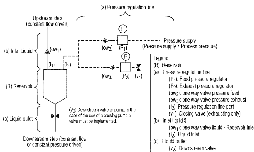
ICPT: Inline Constantly Pressurized Tank - Drawing and Description
