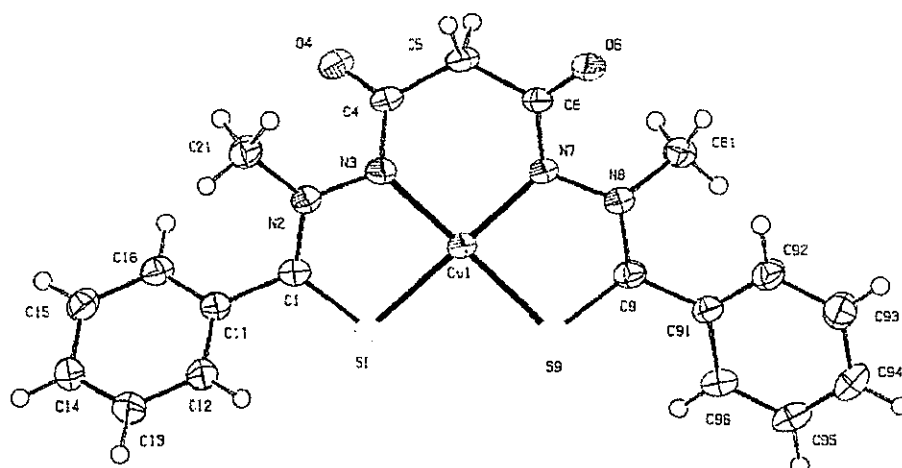
ORTEP diagram of compound 1 showing 50% thermal ellipsoids.
