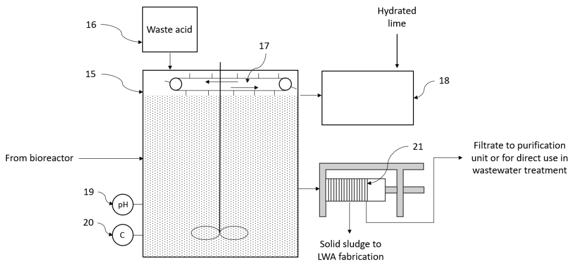
Figure 4: Schematic of coagulant recovery unit
