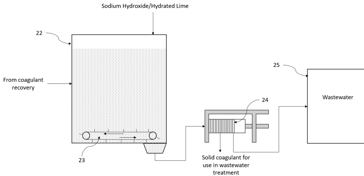
Figure 5: Schematic of purification unit
