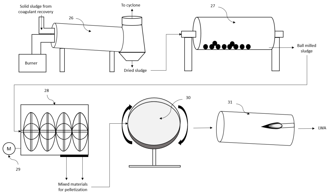
Figure 6: Schematic of lightweight aggregates fabrication unit
