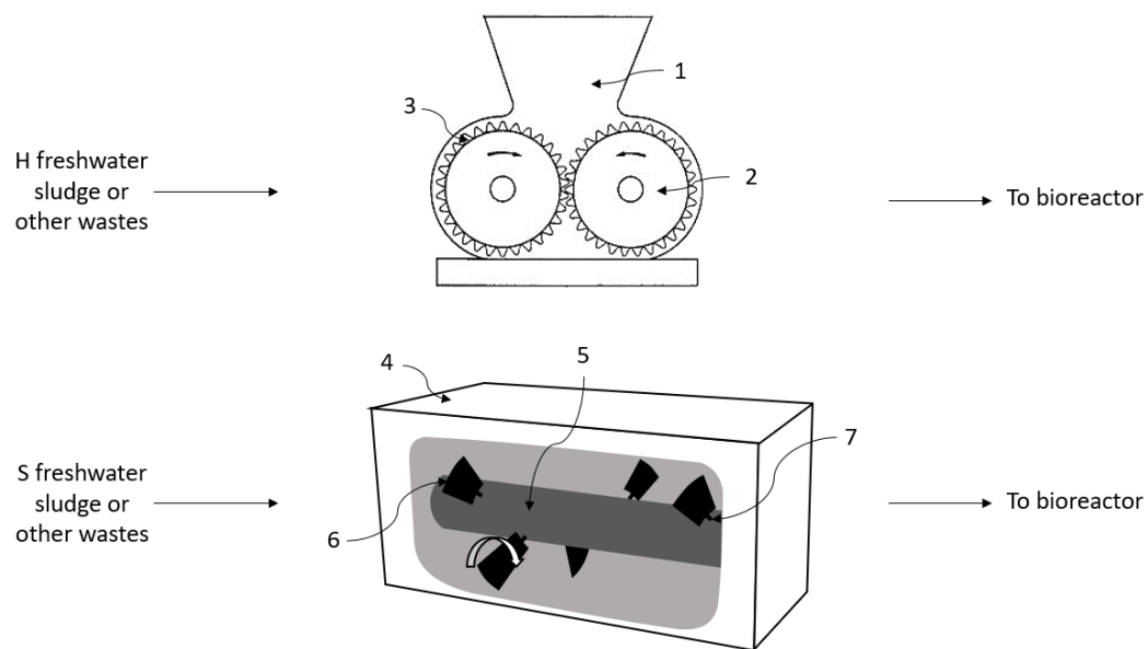
Figure 2: Schematic of pulverization component
