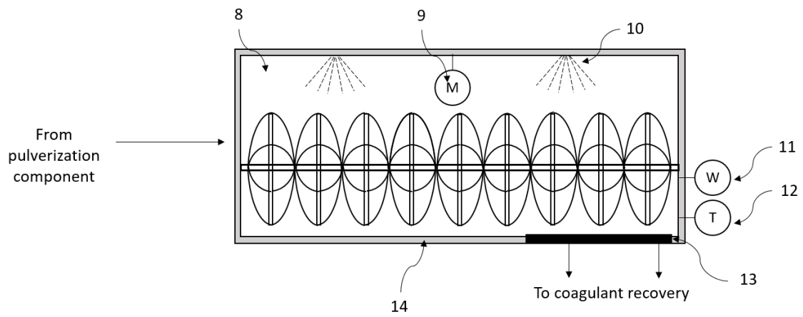
Figure 3: Schematic of bioreactor
