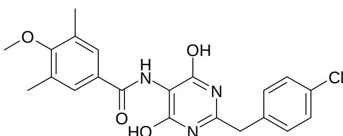
(a) N-[2-(4-Chlorobenzyl)-4,6-dihydroxypyrimidin-5-yl]-4-methoxy-3,5-dimethylbenzamide
