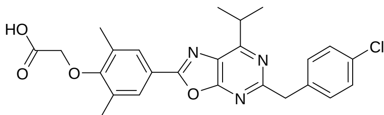
(a) 5-(4-Chlorobenzyl)-7-isopropyl-2-(4-methoxy-3,5-dimethylphenyl)oxazolo[5,4-d]pyrimidine
