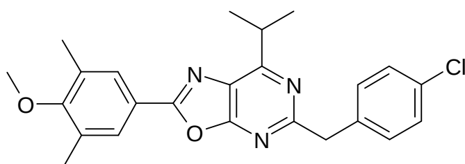
(a) 5-(4-Chlorobenzyl)-7-isopropyl-2-(4-methoxy-3,5-dimethylphenyl)oxazolo[5,4-d]pyrimidine
